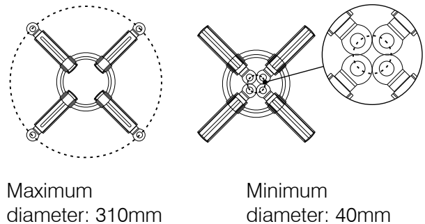
Projector Mounting
