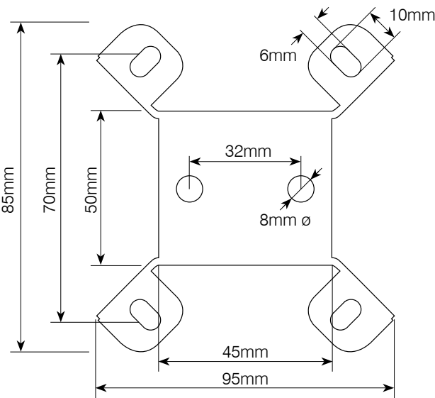
Ceiling Mounting Plate
